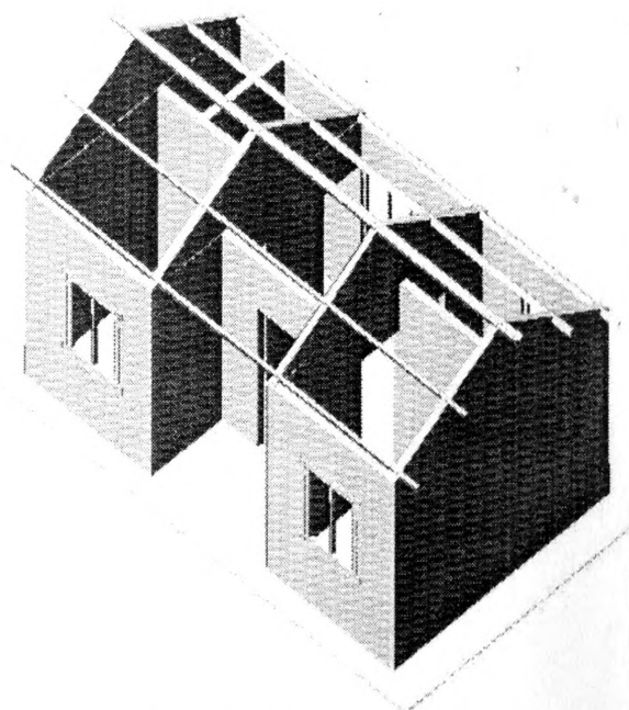
Timber perkins on block gable wall
