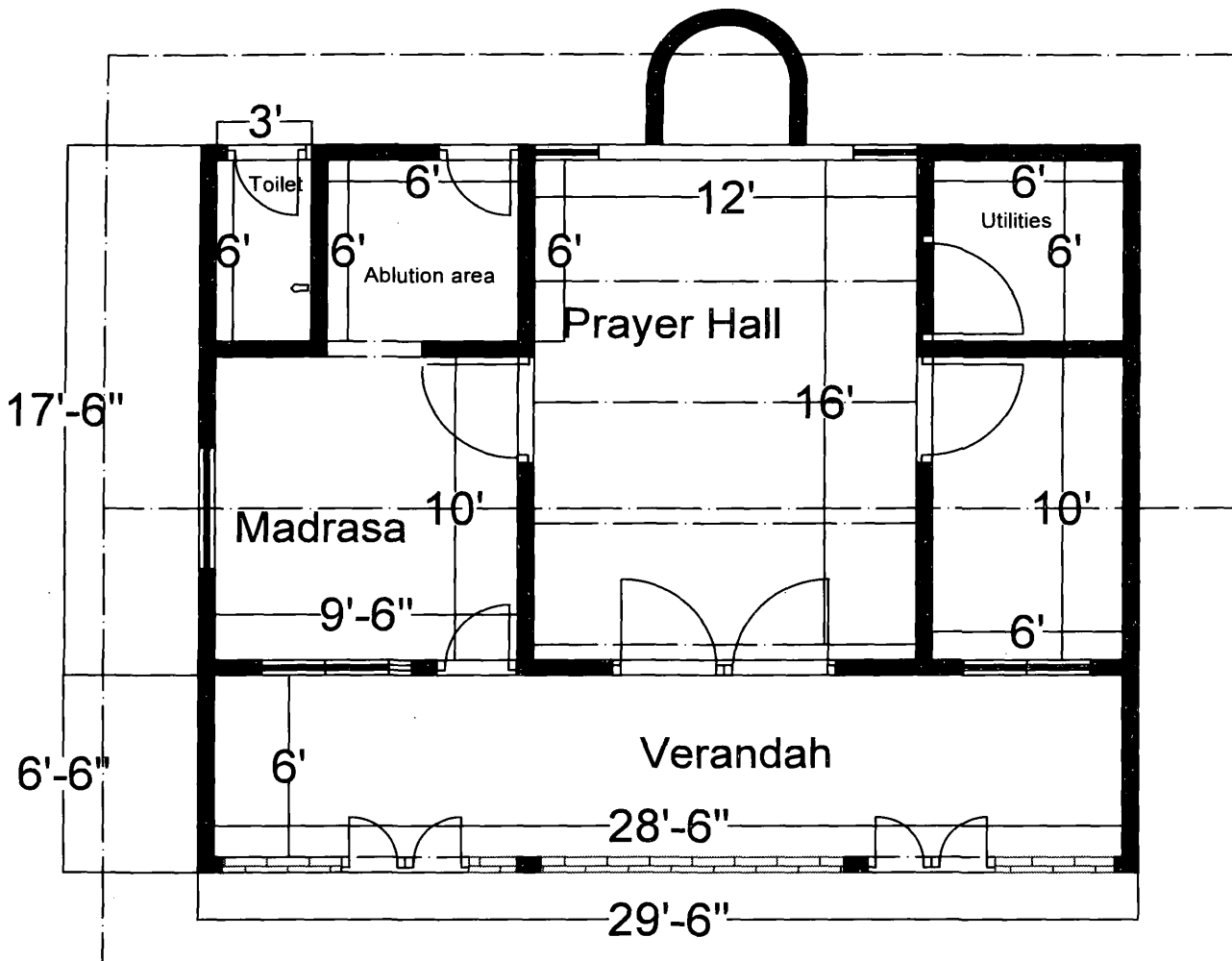
Mosque Plan Floor area 725 sqr.ft
