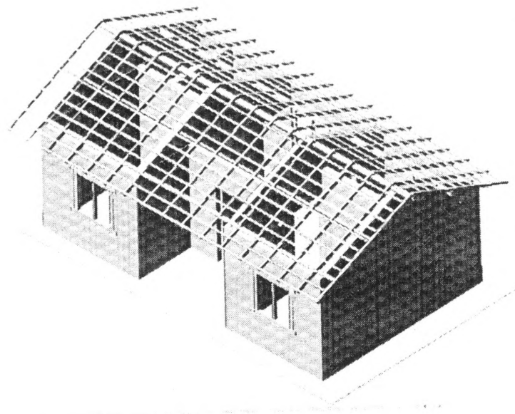
Timber reapers on timber rafters
